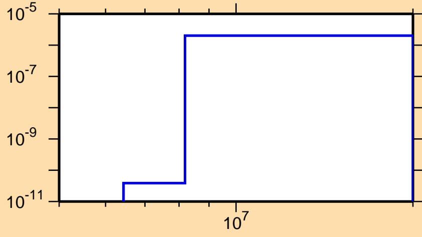
\sigma vs. E for ^{113}\text{Xe}(\text{mt117})
