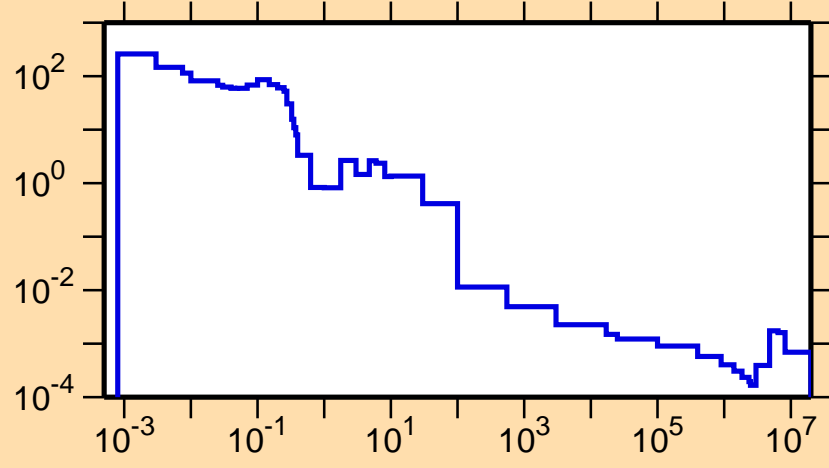
\sigma vs. E for ^{113}\text{Xe}(n,\gamma)
