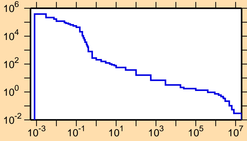
\sigma vs. E for ^{113}\text{Xe}(n,p)
