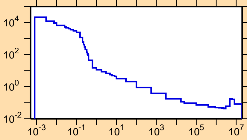
\sigma vs. E for ^{113}\text{Xe}(n,\alpha)
