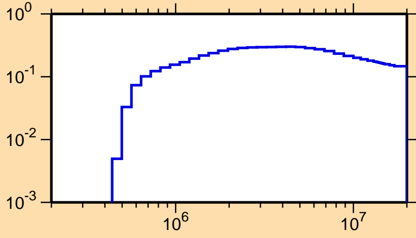
\sigma vs. E for ^{114}\text{Xe}(n,\text{inel.})
