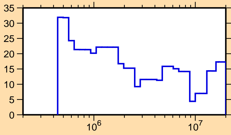
\Delta\sigma/\sigma vs. E for ^{114}\text{Xe}(n,\text{tot.})
