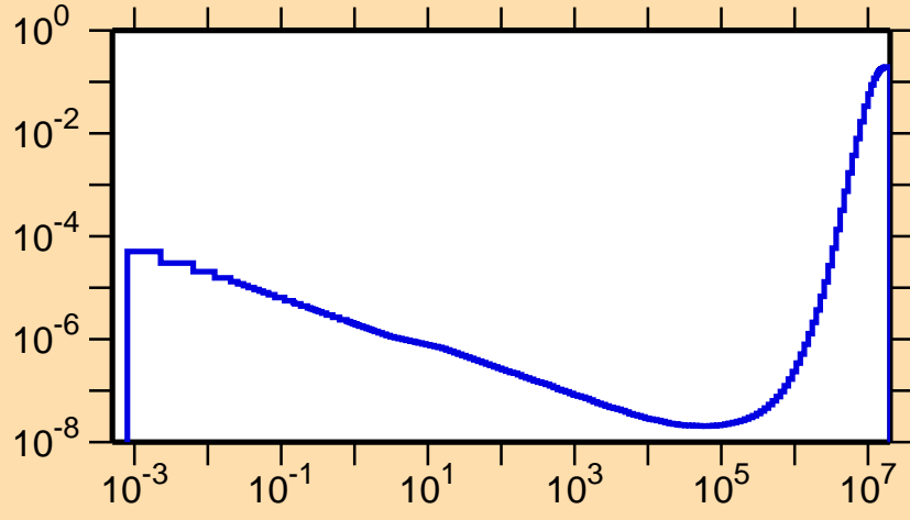
\sigma vs. E for ^{114}\text{Xe}(n,p\alpha)
