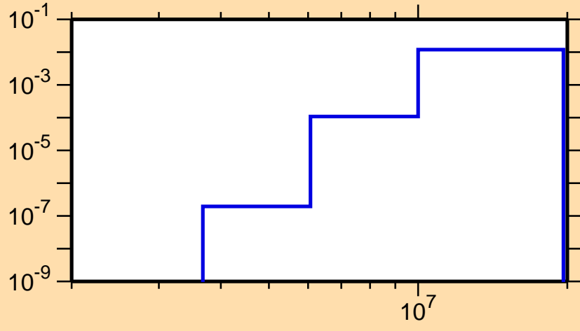
\sigma vs. E for ^{114}\text{Xe}(n,d)
