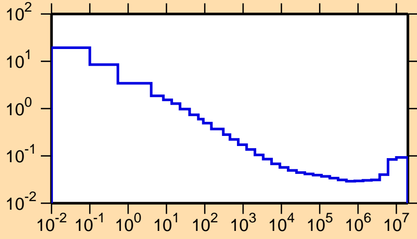
\sigma vs. E for ^{114}\text{Xe}(n,\alpha)
