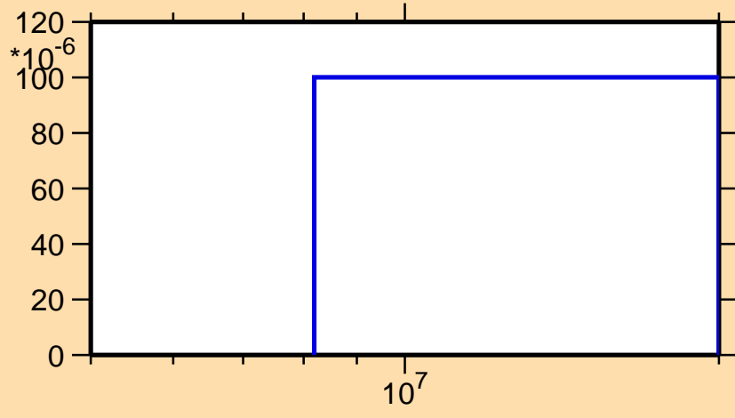
\sigma vs. E for ^{114}\text{Xe}(n,t)
