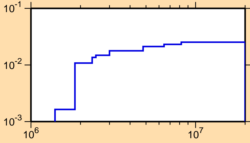
\sigma vs. E for ^{114}\text{Xe}(n,n_4)
