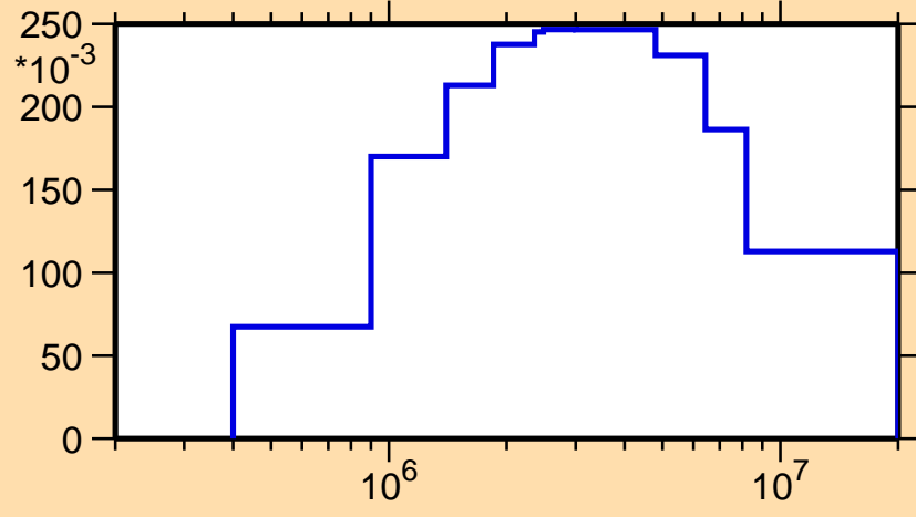
\sigma vs. E for ^{114}\text{Xe}(n,n_1)
