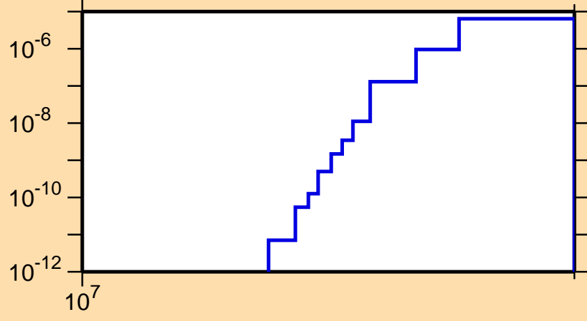
\sigma vs. E for ^{115}\text{Xe}(n,\text{nd})
