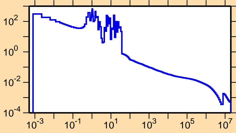
\sigma vs. E for ^{115}\text{Xe}(n,\gamma)
