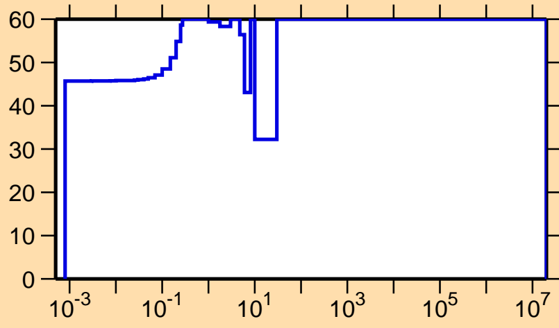
\Delta\sigma/\sigma vs. E for ^{115}\text{Xe}(n,\gamma)
