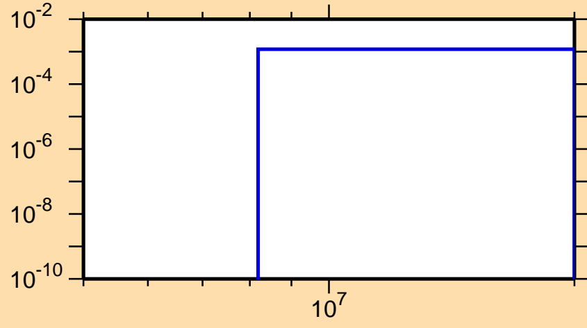
\sigma vs. E for ^{115}\text{Xe}(n,\text{pd})
