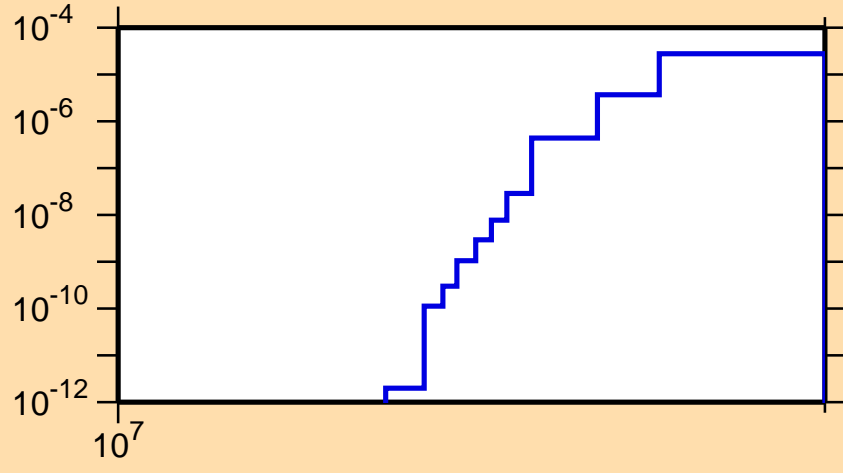
\sigma vs. E for ^{117}\text{Xe}(n,nd)
