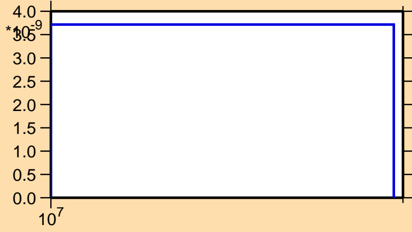
\sigma vs. E for ^{117}\text{Xe} (mt 34)
