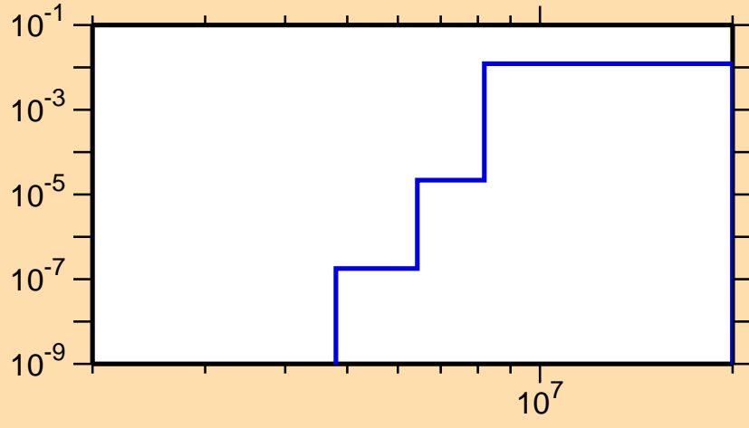
\sigma vs. E for ^{117}\text{Xe}(n,d)
