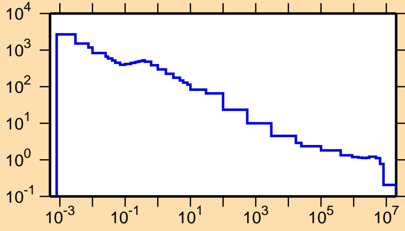
\sigma vs. E for ^{117}\text{Xe}(n,p)
