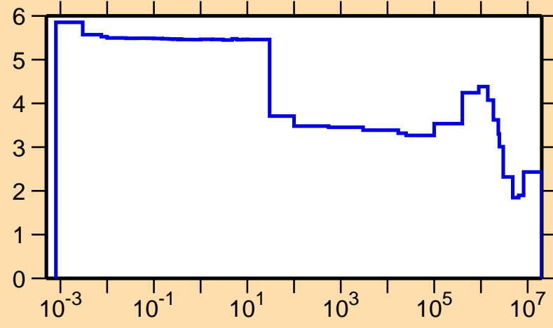
\sigma vs. E for ^{117}\text{Xe}(n,\text{el.})
