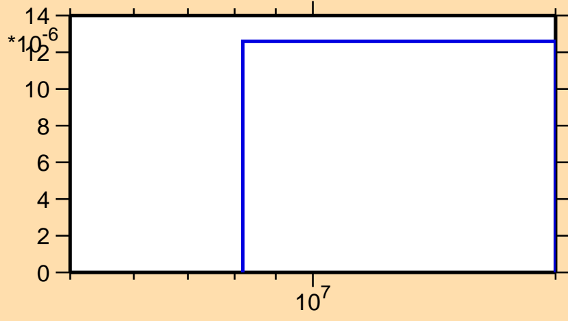
\sigma vs. E for ^{117}\text{Xe}(\text{mt } 45)
