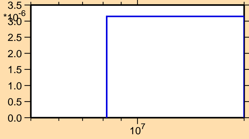
\sigma vs. E for ^{117}\text{Xe}(n,\text{pt})
