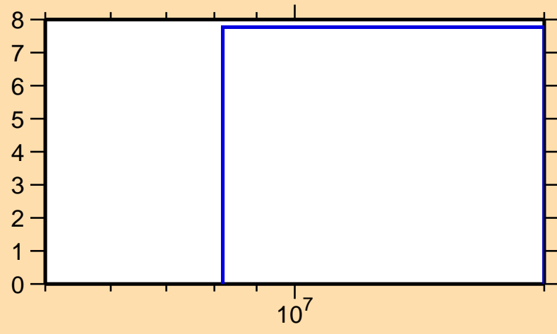
\Delta\sigma/\sigma vs. E for ^{117}\text{Xe}(n,\text{nonel.})
