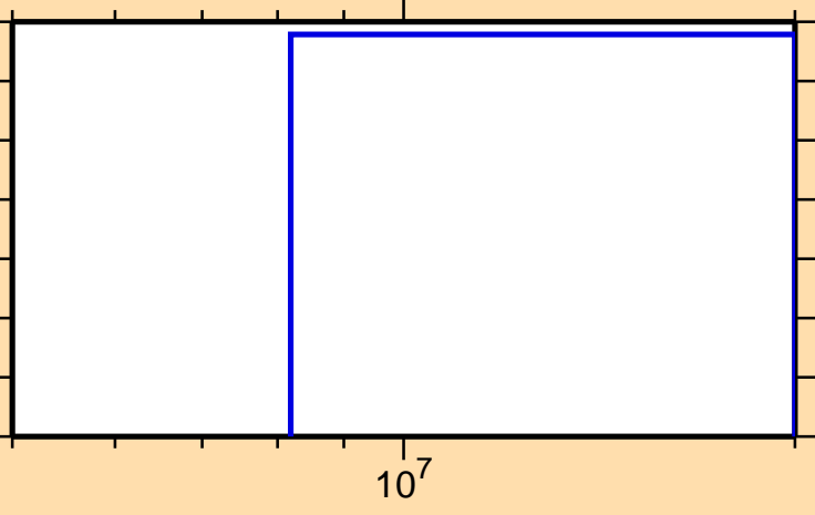
\sigma vs. E for ^{117}\text{Xe}(n,\text{pd})
