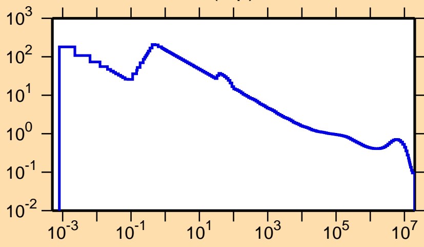
\sigma vs. E for ^{119}\text{Xe}(n,p)
