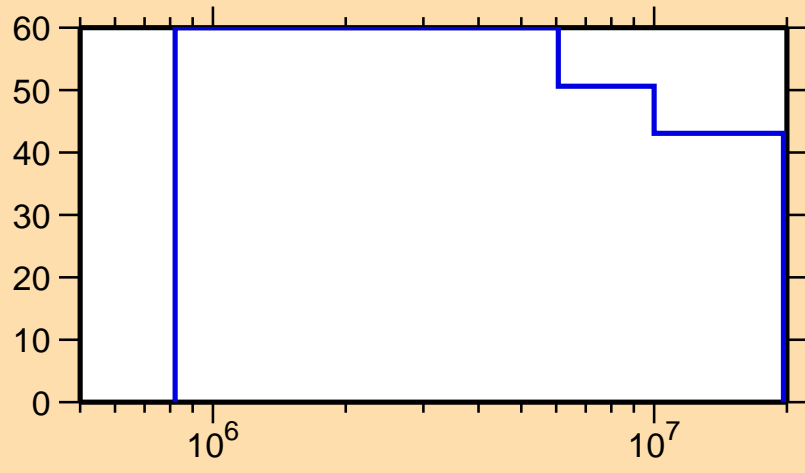
\Delta\sigma/\sigma vs. E for ^{119}\text{Xe}(n,n\text{cont.})
