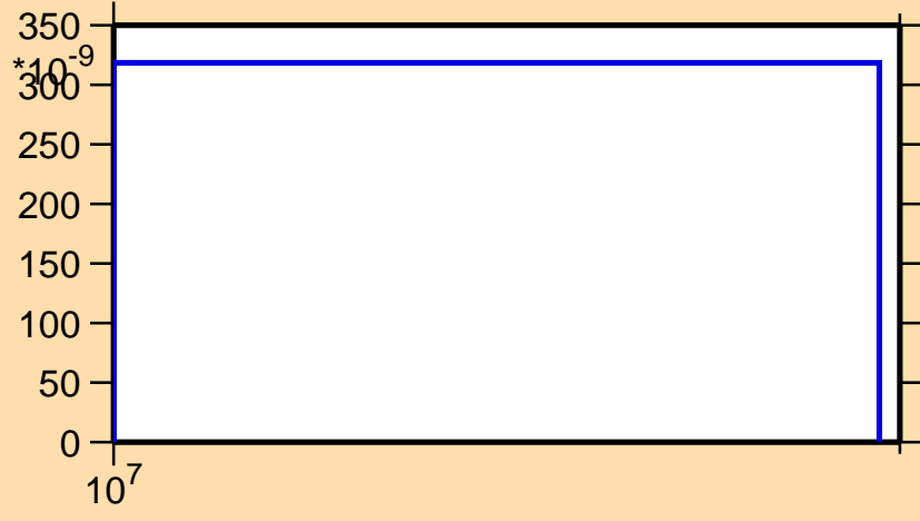
\sigma vs. E for ^{119}\text{Xe} (mt 45)
