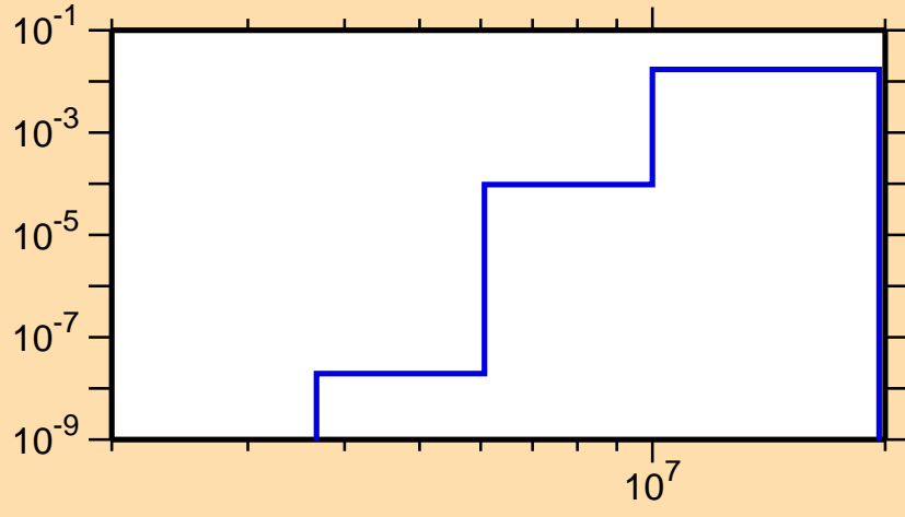
\sigma vs. E for ^{119}\text{Xe}(n,n\alpha)
