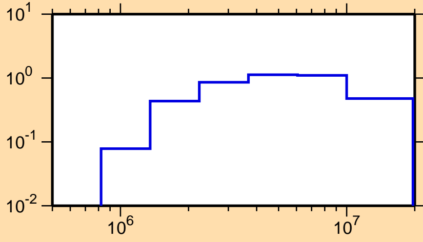
\sigma vs. E for ^{119}\text{Xe}(n,n\text{cont.})
