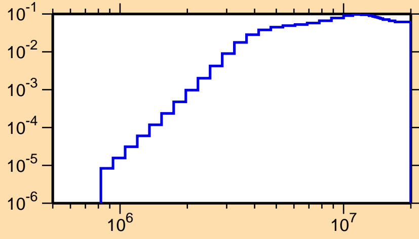
\sigma vs. E for ^{122}\text{Xe}(n,p)
