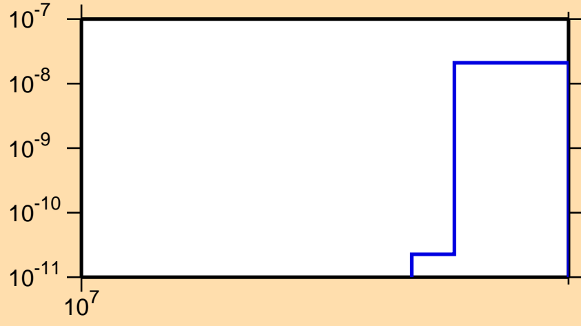
\sigma vs. E for ^{122}\text{Xe}(n,2n\alpha)
