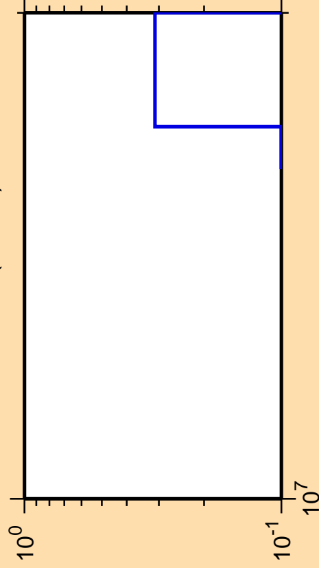
\Delta\sigma/\sigma vs. E for ^{122}\text{Xe} (mt 34)
