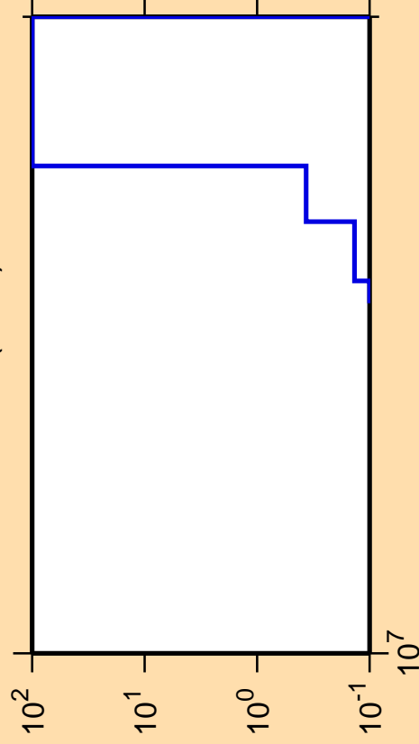
\Delta\sigma/\sigma vs. E for ^{122}\text{Xe}(n,nd)
