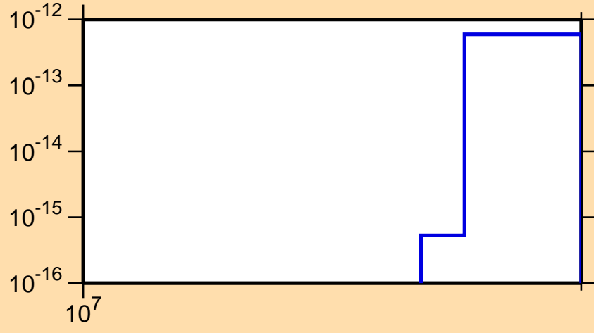
\sigma vs. E for ^{122}\text{Xe}(n,nt)
