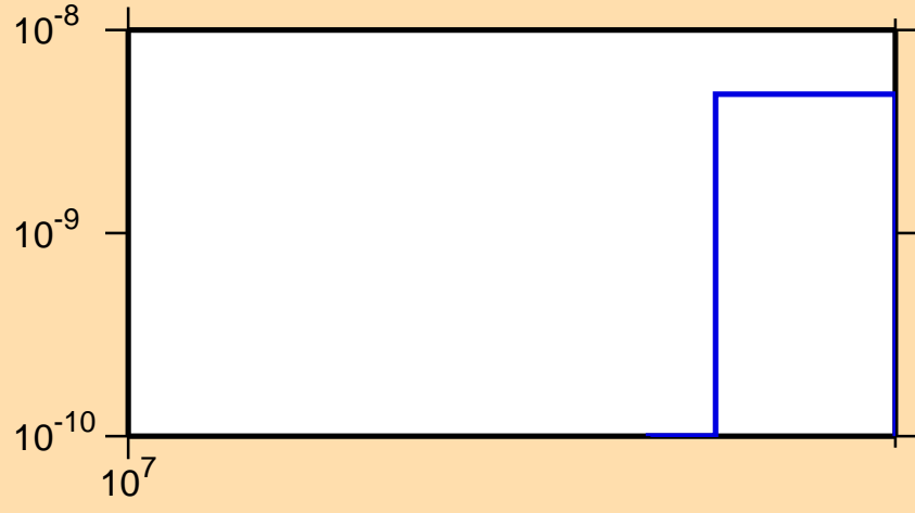
\sigma vs. E for ^{122}\text{Xe} (mt 45)
