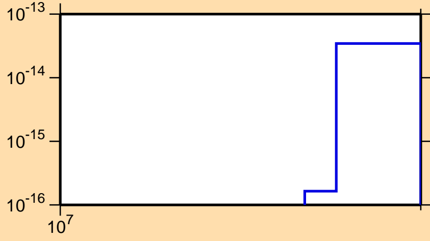
\sigma vs. E for ^{122}\text{Xe} (mt 34)
