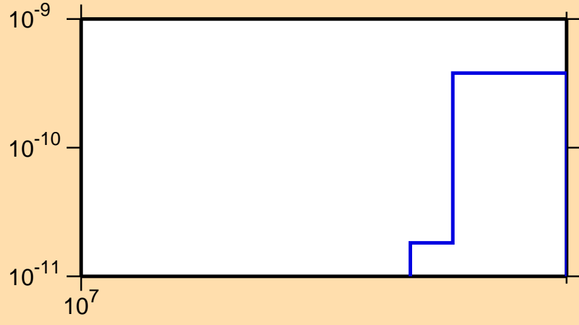
\sigma vs. E for ^{122}\text{Xe}(\text{mt117})
