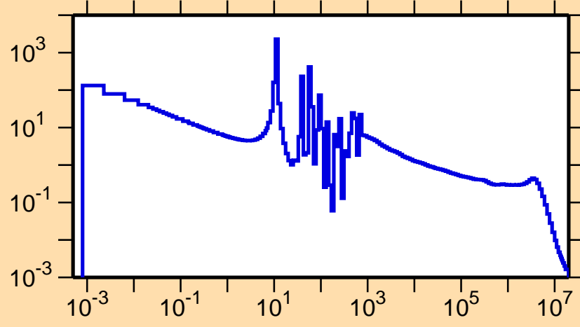
\sigma vs. E for ^{122}\text{Xe}(n,\gamma)
