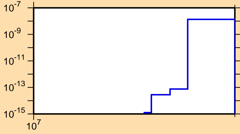
\sigma vs. E for ^{122}\text{Xe}(n,nd)
