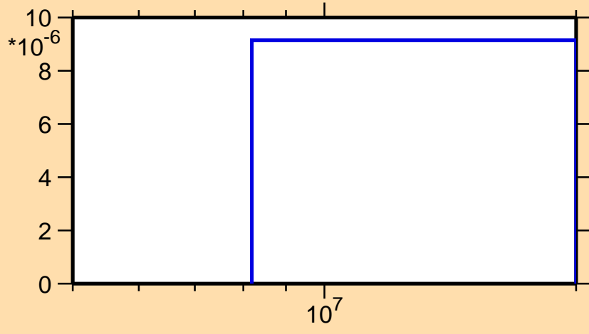
\sigma vs. E for ^{122}\text{Xe}(n,t)
