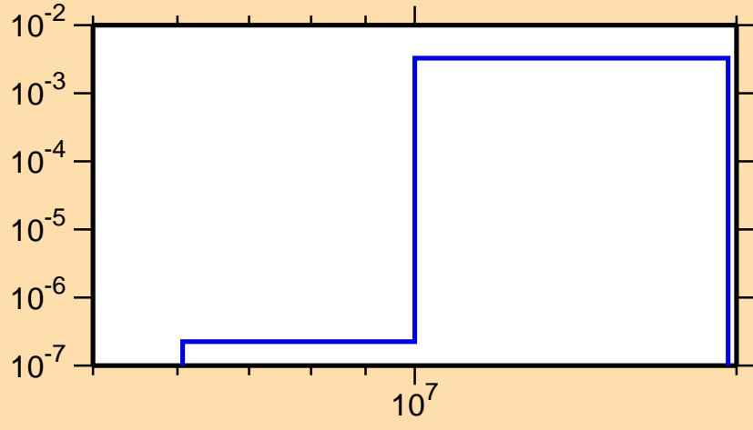
\sigma vs. E for ^{123}\text{Xe}(n,d)
