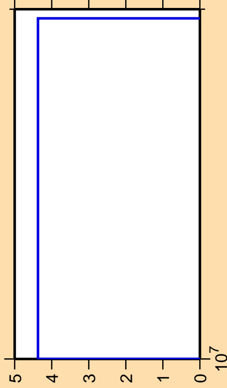
\Delta\sigma/\sigma vs. E for ^{123}\text{Xe} (mt 45)
