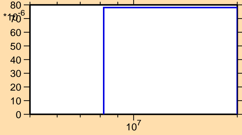
\sigma vs. E for ^{123}\text{Xe}(n,t)
