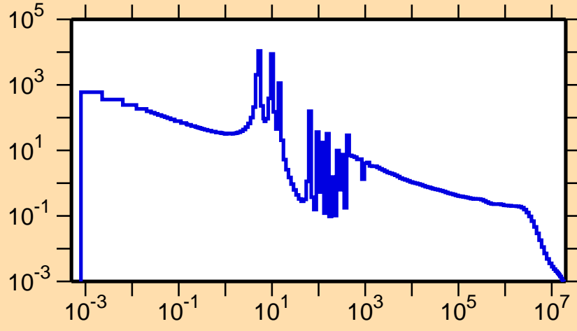
\sigma vs. E for ^{124}\text{Xe}(n,\gamma)
