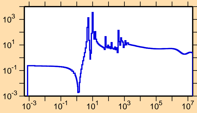
\sigma vs. E for ^{124}\text{Xe}(n,\text{el.})
