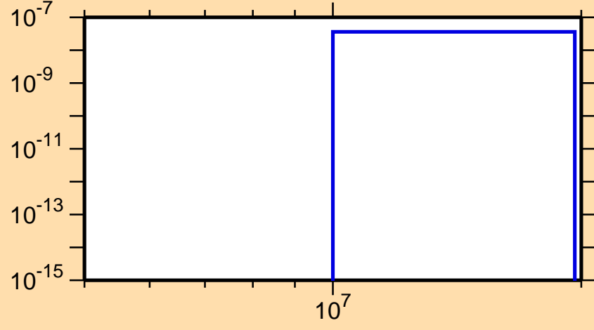
\sigma vs. E for ^{124}\text{Xe}(n,\text{He}3)
