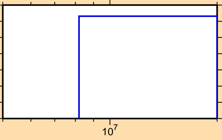
\sigma vs. E for ^{124}\text{Xe}(n,3n)
