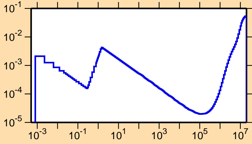
\sigma vs. E for ^{125}\text{Xe}(n,p)
