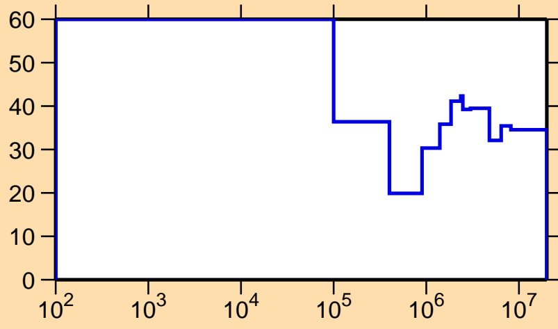
\Delta\sigma/\sigma vs. E for ^{125}\text{Xe}(n,n_1)
