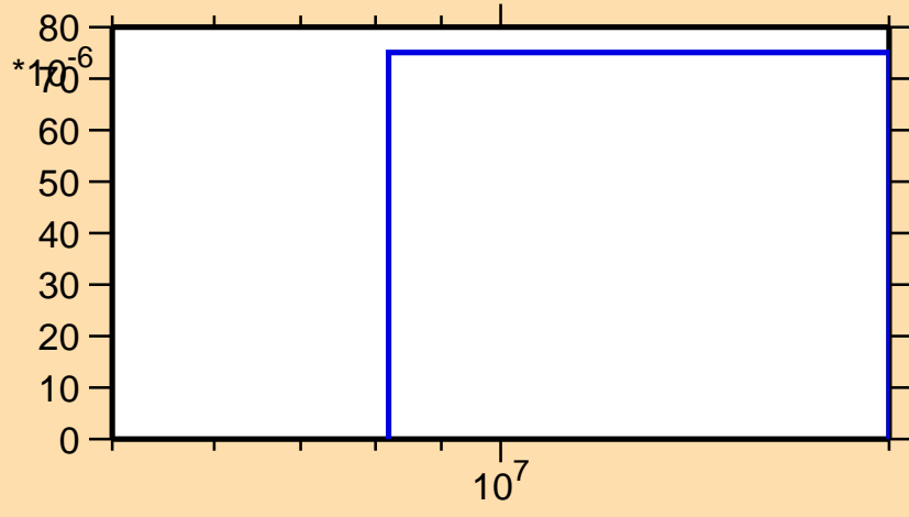
\sigma vs. E for ^{125}\text{Xe}(n,t)
