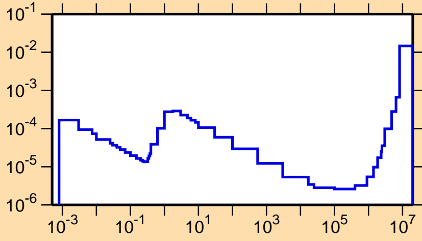
\sigma vs. E for ^{125}\text{Xe}(n,\alpha)
