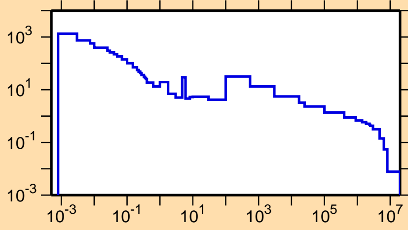
\sigma vs. E for ^{125}\text{Xe}(n,\gamma)
