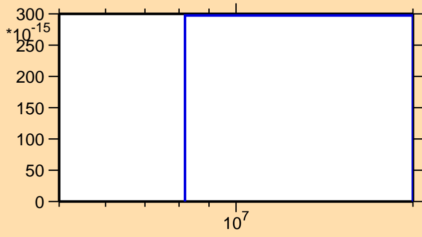
\sigma vs. E for ^{125}\text{Xe}(n,\text{pt})
