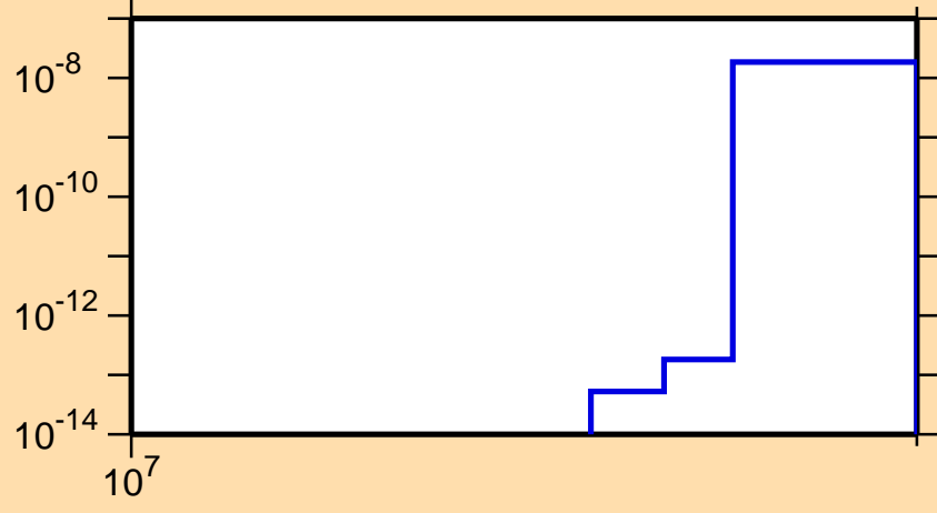
\sigma vs. E for ^{126}\text{Xe}(n,nd)
