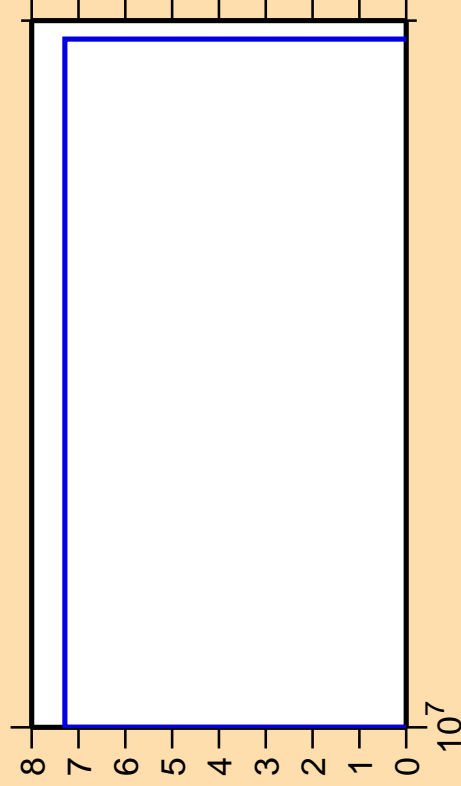
\Delta\sigma/\sigma vs. E for ^{126}\text{Xe}(n,pd)
