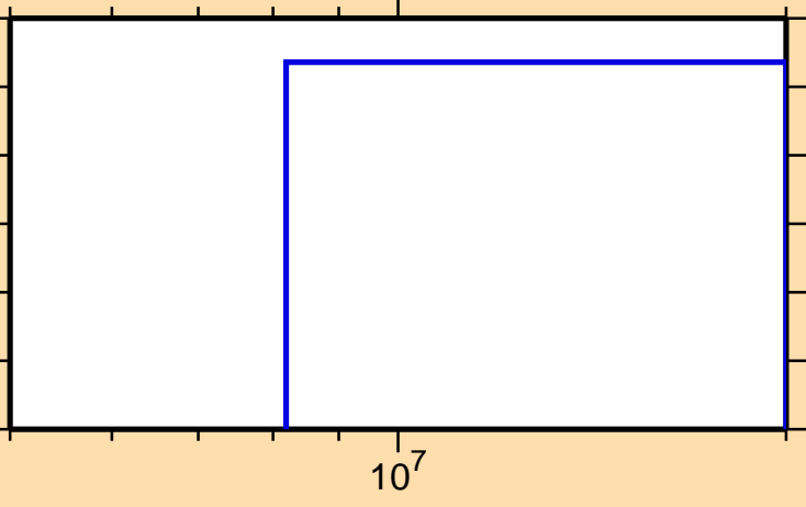
\sigma vs. E for ^{127}\text{Xe}(\text{mt } 34)
