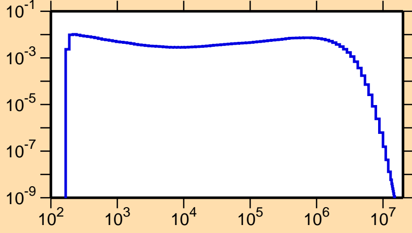
\sigma vs. E for ^{127}\text{Xe}(n,n_1)
