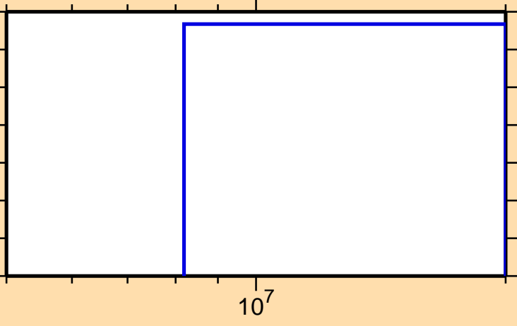
\sigma vs. E for ^{127}\text{Xe}(n,p\alpha)
