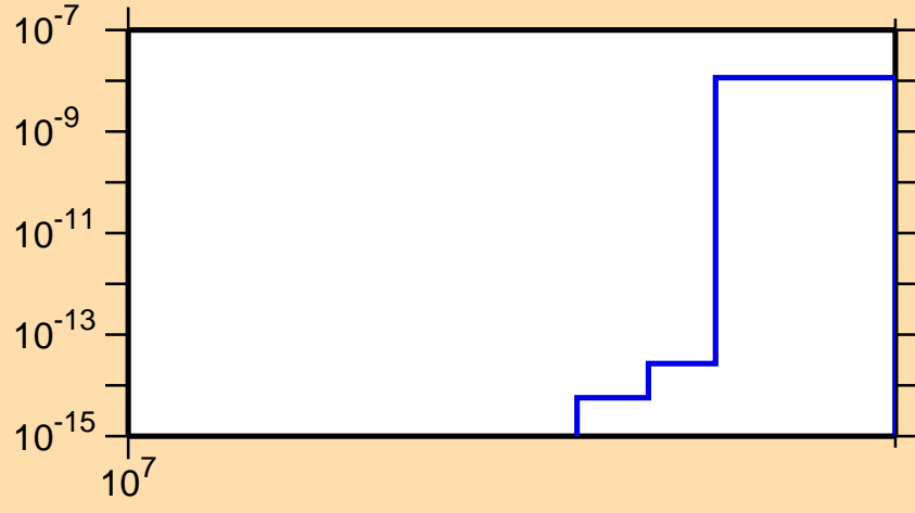
\sigma vs. E for ^{128}\text{Xe}(n,\text{nd})
