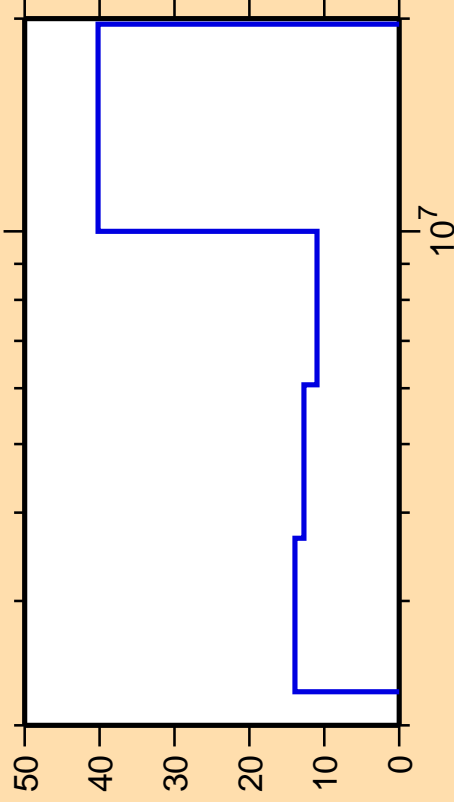
\Delta\sigma/\sigma vs. E for ^{128}\text{Xe}(n,n\text{cont.})
