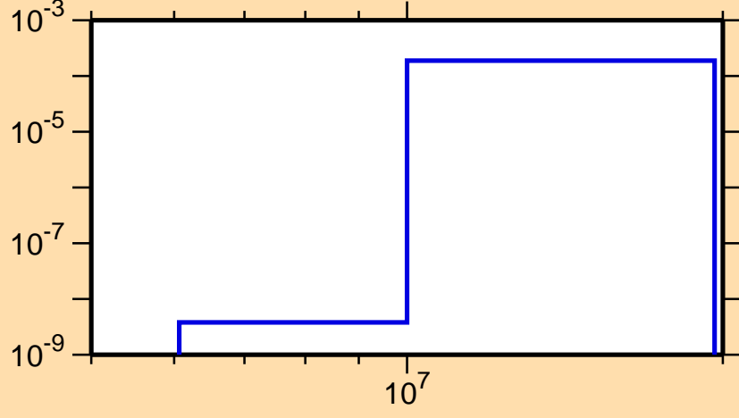
\sigma vs. E for ^{128}\text{Xe}(n,n\alpha)
