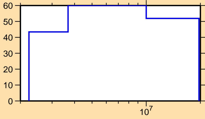
\Delta\sigma/\sigma vs. E for ^{128}\text{Xe}(n,p)
