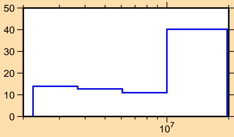
\Delta\sigma/\sigma vs. E for ^{128}\text{Xe}(n,n\text{cont.})
