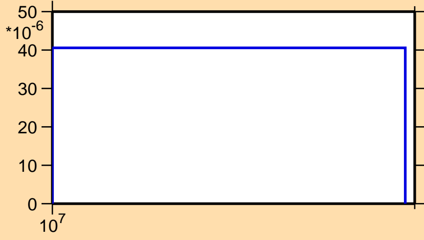
\sigma vs. E for ^{128}\text{Xe}(n,3n)
