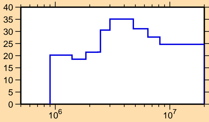
\Delta\sigma/\sigma vs. E for ^{128}\text{Xe}(n,n_1)
