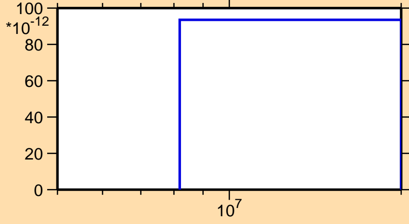
\sigma vs. E for ^{128}\text{Xe}(n,\text{nd})
