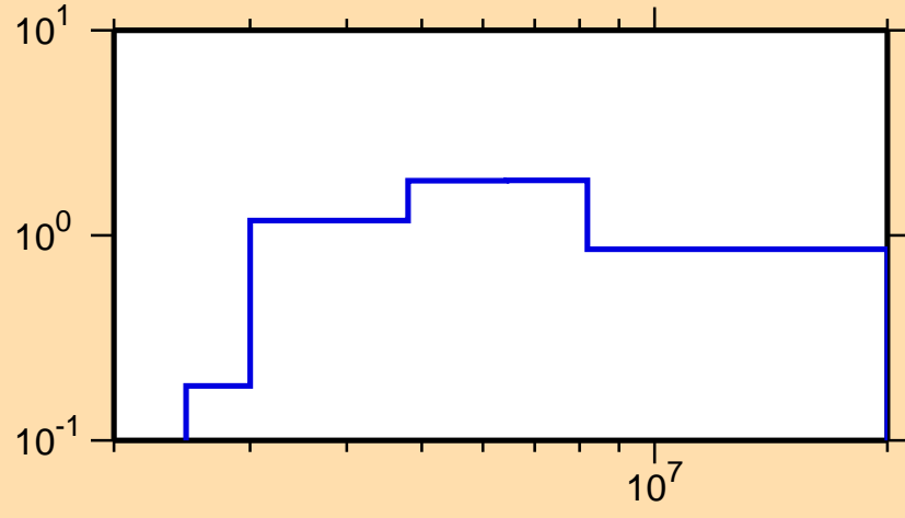
\sigma vs. E for ^{128}\text{Xe}(n,n\text{cont.})
