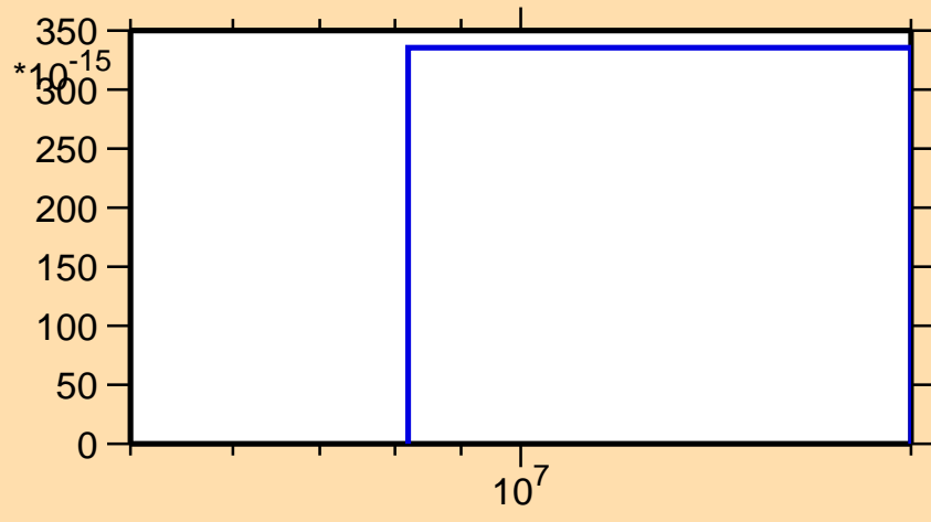
\sigma vs. E for ^{128}\text{Xe}(n,nt)
