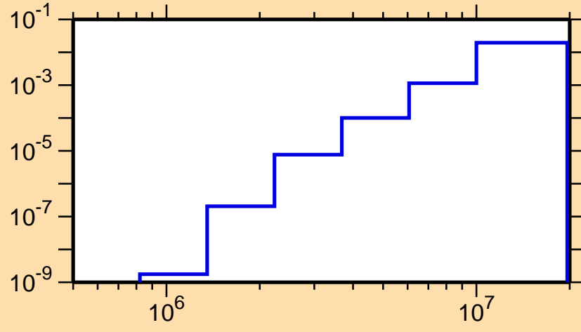
\sigma vs. E for ^{129}\text{Xe}(n,p)
