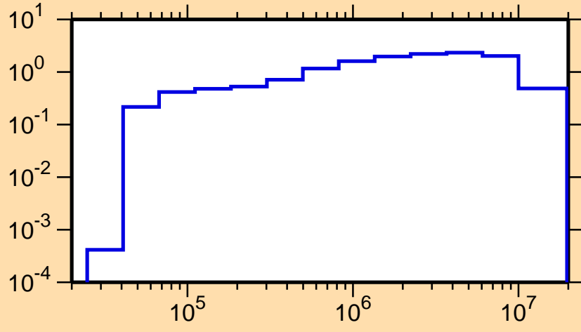
\sigma vs. E for ^{129}\text{Xe}(n,\text{inel.})
