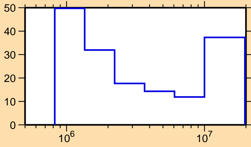
\Delta\sigma/\sigma vs. E for ^{129}\text{Xe}(n,n\text{cont.})
