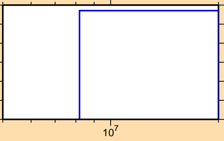
\sigma vs. E for ^{129}\text{Xe}(n,\text{nd})
