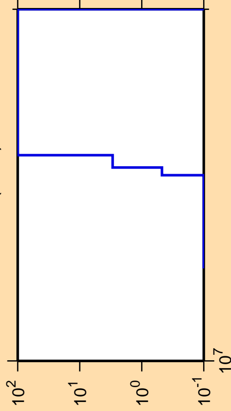
\Delta\sigma/\sigma vs. E for ^{129}\text{Xe}(n,nd)
