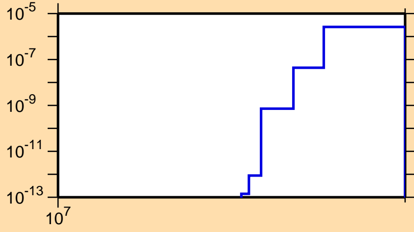
\sigma vs. E for ^{129}\text{Xe}(n,nd)
