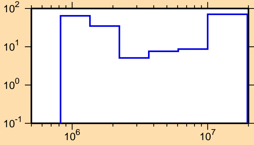
\Delta\sigma/\sigma vs. E for ^{129}\text{Xe}(n,n\text{cont.})
