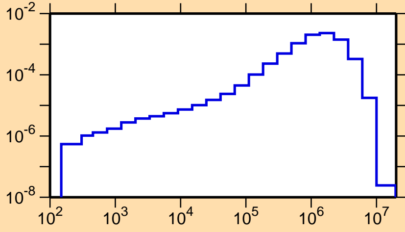
\sigma vs. E for ^{129}\text{Xe}(n,n_1)
