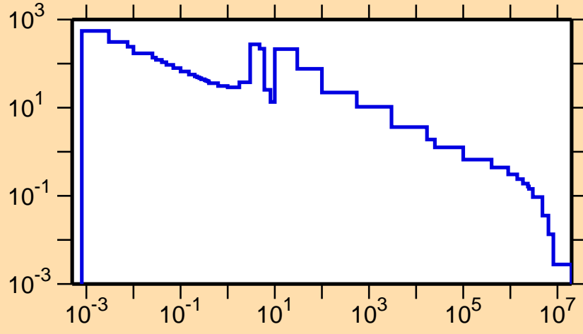
\sigma vs. E for ^{129}\text{Xe}(n,\gamma)
