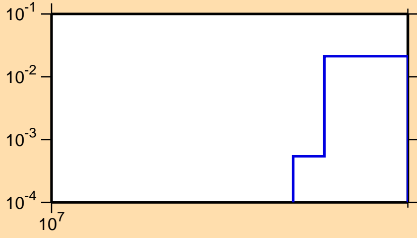
\sigma vs. E for ^{130}\text{Xe}(n,3n)
