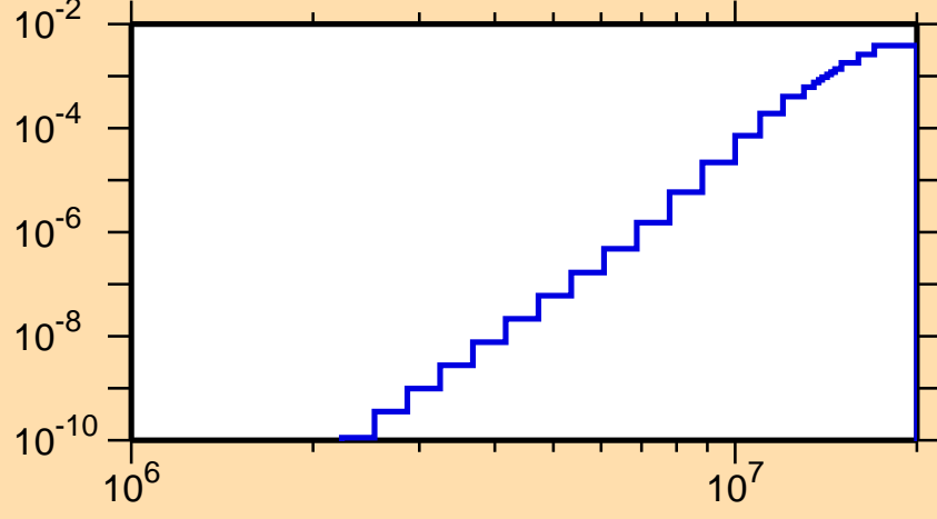
\sigma vs. E for ^{130}\text{Xe}(n,\alpha)
