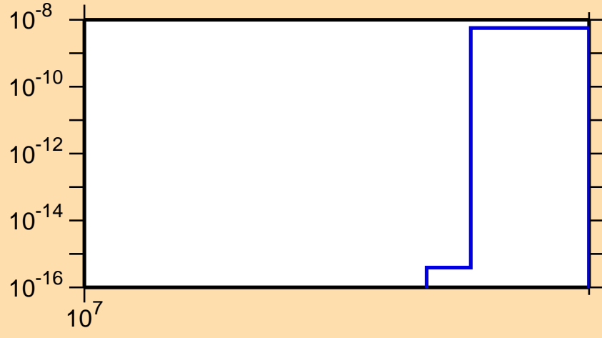
\sigma vs. E for ^{130}\text{Xe}(n,\text{nd})
