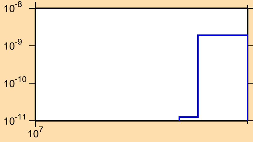
\sigma vs. E for ^{130}\text{Xe}(n,\text{He}3)
