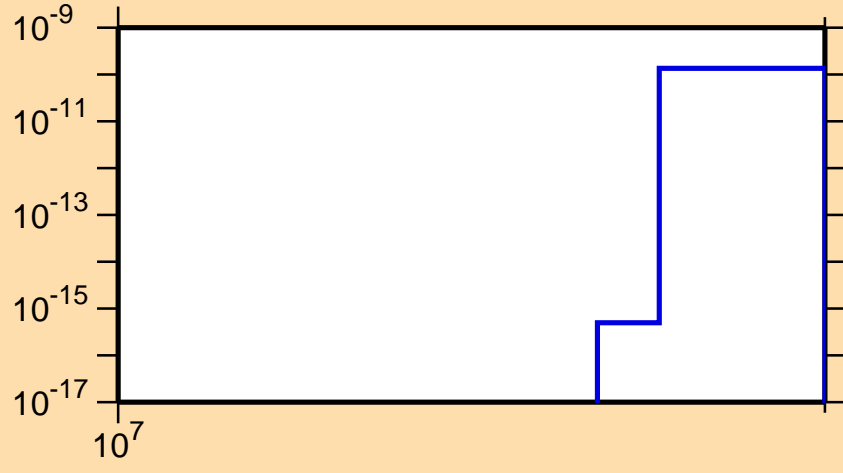
\sigma vs. E for ^{130}\text{Xe}(n,nt)
