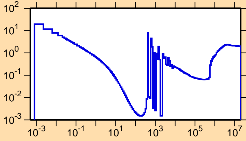
\sigma vs. E for ^{130}\text{Xe}(n,\text{nonel.})
