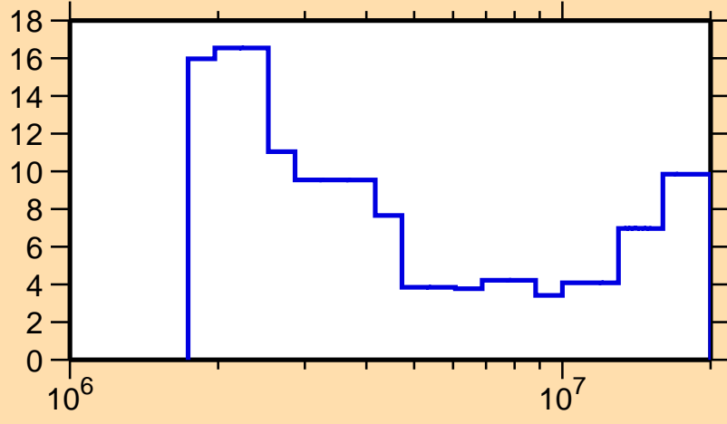
\Delta\sigma/\sigma vs. E for ^{130}\text{Xe}(n,\text{tot.})
