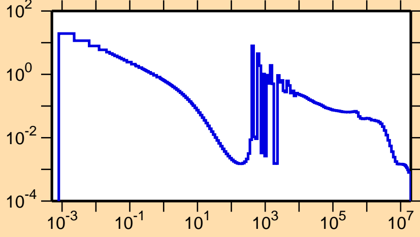
\sigma vs. E for ^{130}\text{Xe}(n,\gamma)
