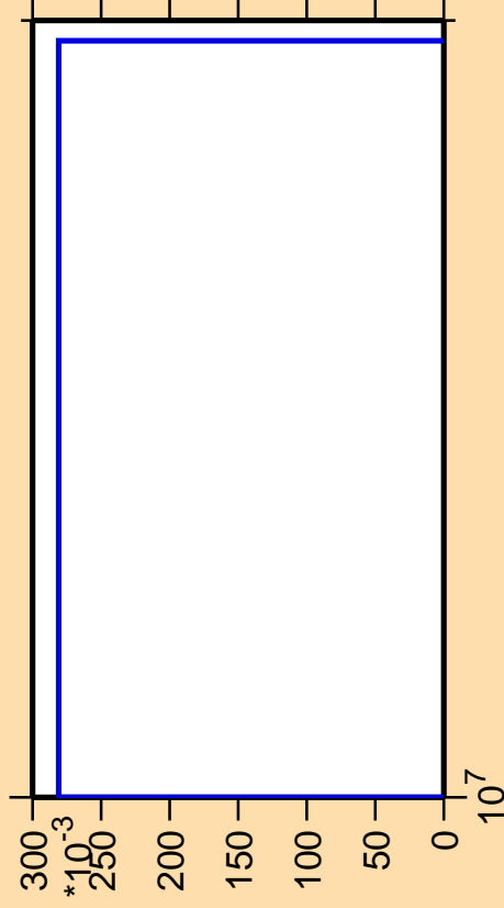
\Delta\sigma/\sigma vs. E for ^{130}\text{Xe}(n,2np)
