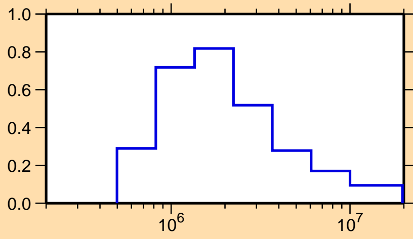
\sigma vs. E for ^{130}\text{Xe}(n,n_1)
