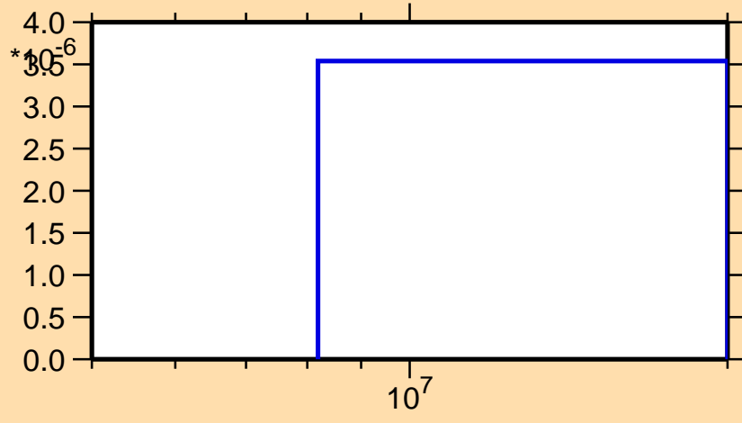
\sigma vs. E for ^{130}\text{Xe}(n,t)
