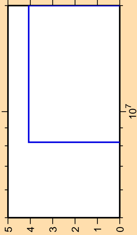
\Delta\sigma/\sigma vs. E for ^{130}\text{Xe}(n,nt)
