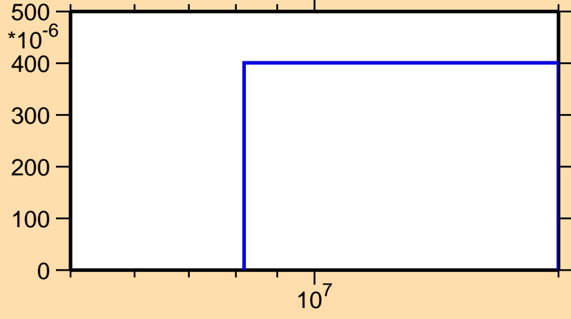
\sigma vs. E for ^{130}\text{Xe}(n,np)
