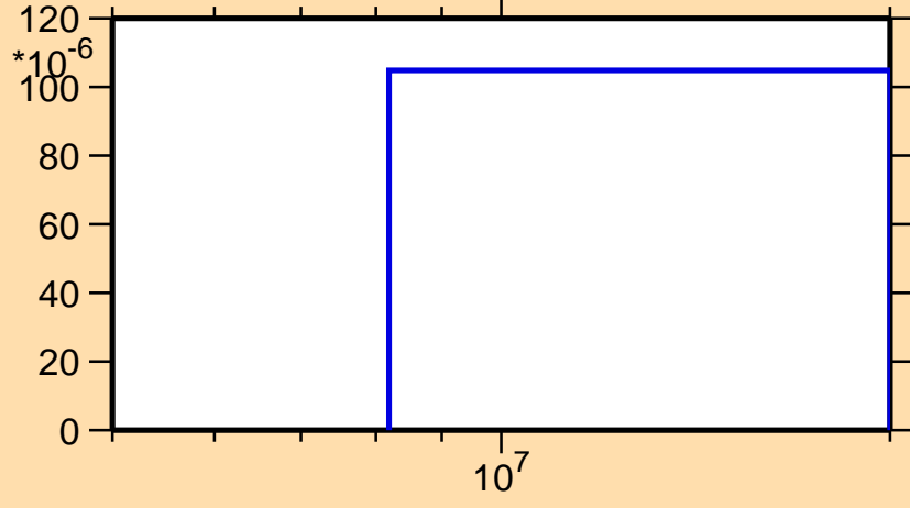
\sigma vs. E for ^{131}\text{Xe}(n,np)
