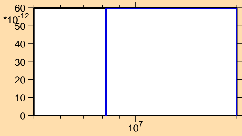
\sigma vs. E for ^{131}\text{Xe}(n,2n\alpha)
