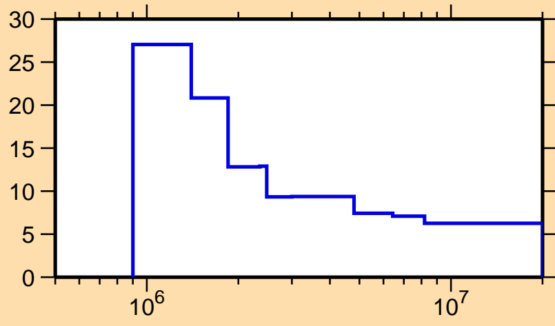
\Delta\sigma/\sigma vs. E for ^{131}\text{Xe}(n,\text{nonel.})
