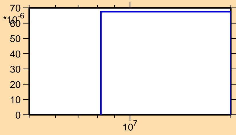
\sigma vs. E for ^{131}\text{Xe}(n,t)
