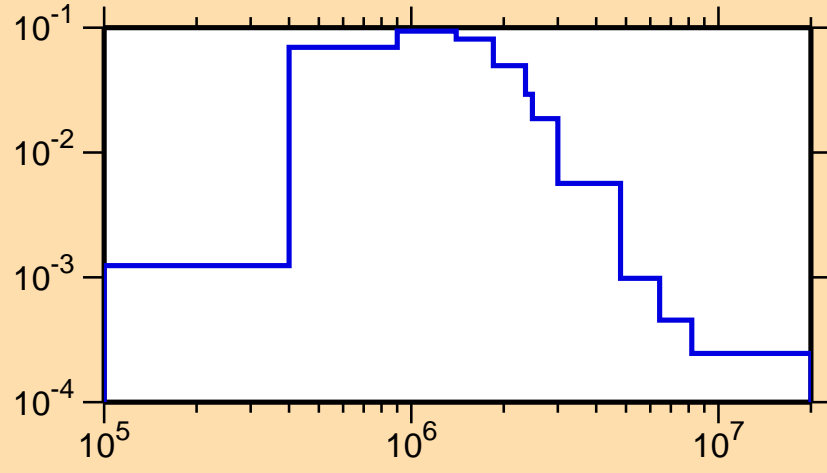
\sigma vs. E for ^{131}\text{Xe}(n,n_3)
