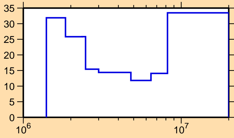
\Delta\sigma/\sigma vs. E for ^{131}\text{Xe}(n,n\text{cont.})
