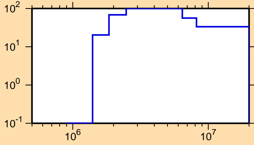
\Delta\sigma/\sigma vs. E for ^{131}\text{Xe}(n,p)
