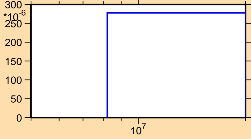
\sigma vs. E for ^{131}\text{Xe}(n,d)
