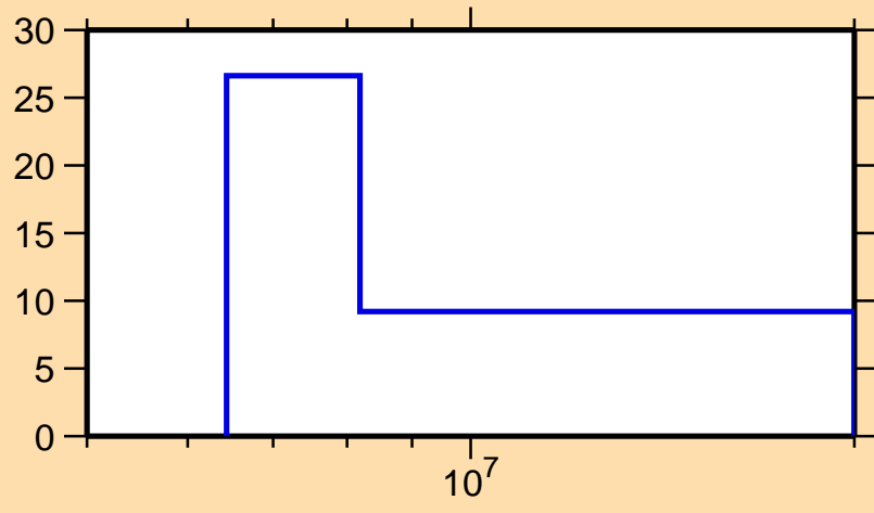
\Delta\sigma/\sigma vs. E for ^{131}\text{Xe}(n,2n)
