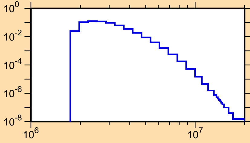
\sigma vs. E for ^{132}\text{Xe}(n,n_4)
