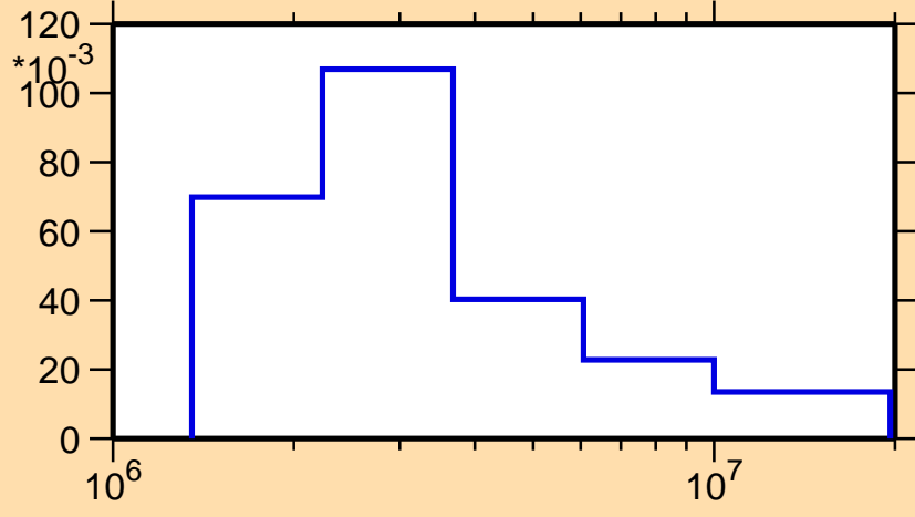
\sigma vs. E for ^{132}\text{Xe}(n,n_3)
