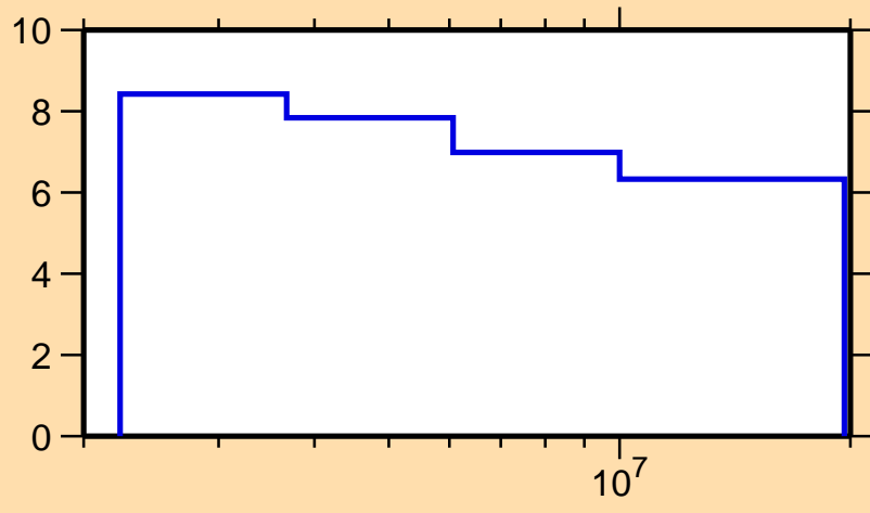
\Delta\sigma/\sigma vs. E for ^{132}\text{Xe}(n,n\text{onel.})
