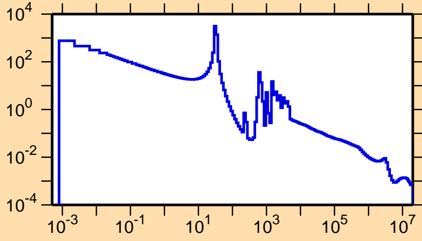
\sigma vs. E for ^{133}\text{Xe}(n,\gamma)
