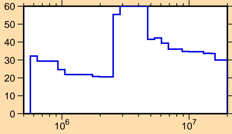
\Delta\sigma/\sigma vs. E for ^{133}\text{Xe}(n,n_1)
