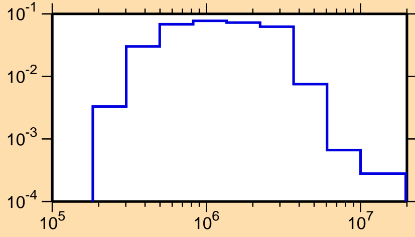
\sigma vs. E for ^{133}\text{Xe}(n,n_1)
