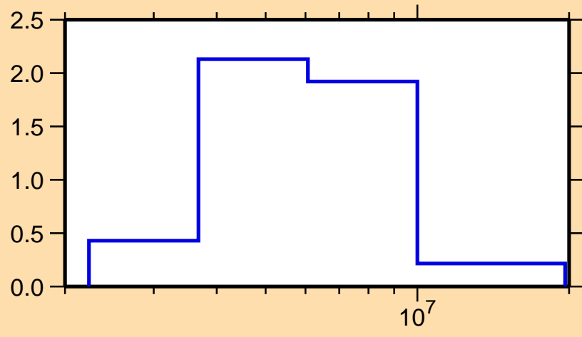
\sigma vs. E for ^{133}\text{Xe}(n,n\text{cont.})
