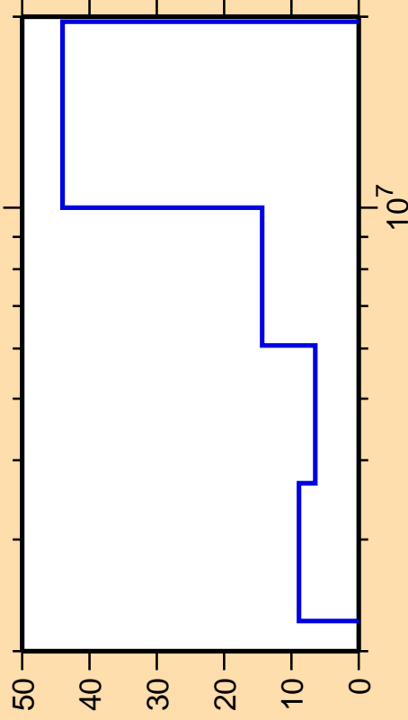
\Delta\sigma/\sigma vs. E for ^{133}\text{Xe}(n,n\text{cont.})
