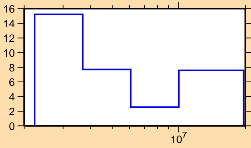
\Delta\sigma/\sigma vs. E for ^{133}\text{Xe}(n,\text{tot.})
