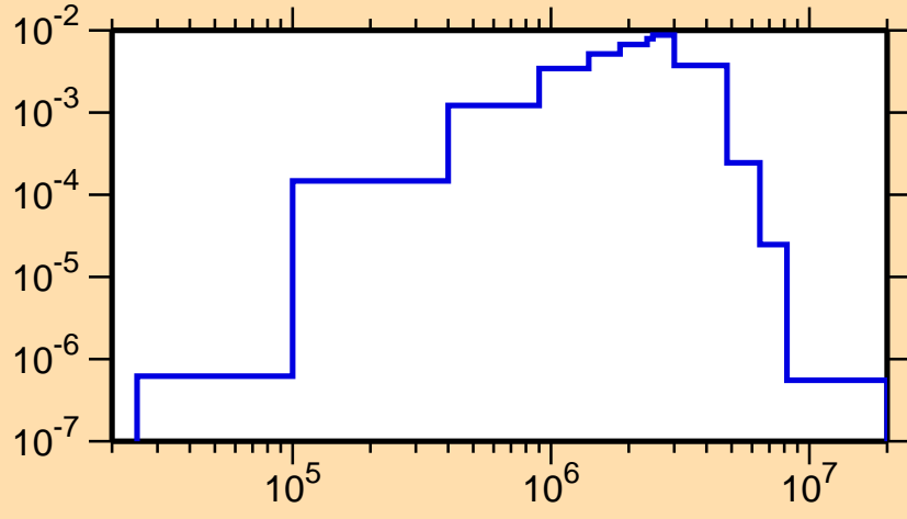
\sigma vs. E for ^{133}\text{Xe}(n,n_2)
