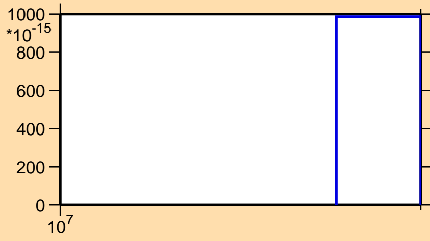
\sigma vs. E for ^{134}\text{Xe}(n,2np)
