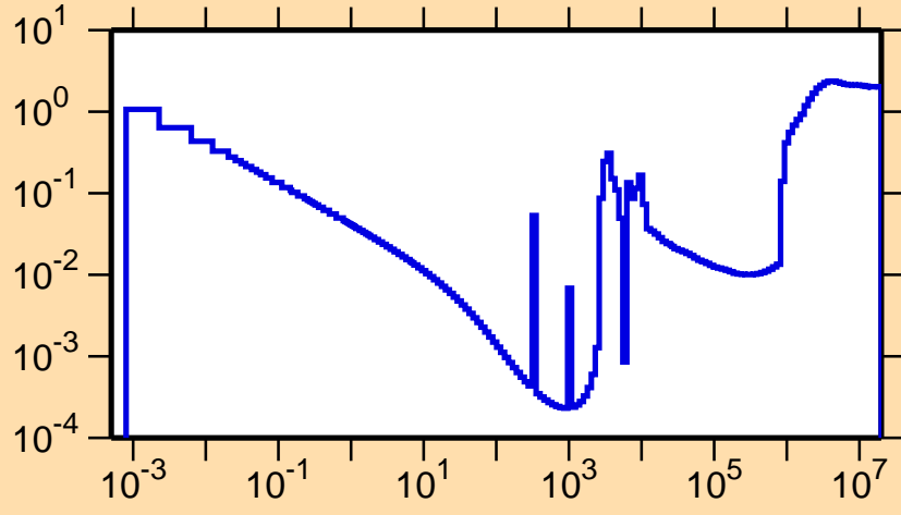
\sigma vs. E for ^{134}\text{Xe}(n,\text{nonel.})
