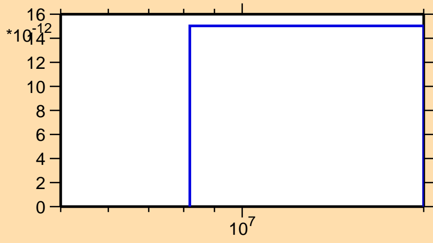
\sigma vs. E for ^{134}\text{Xe}(n,\text{nd})
