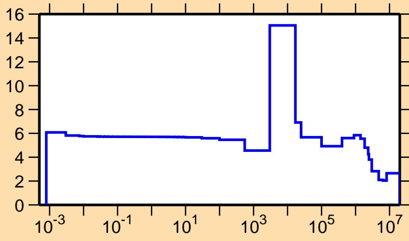
\sigma vs. E for ^{134}\text{Xe}(n,\text{el.})
