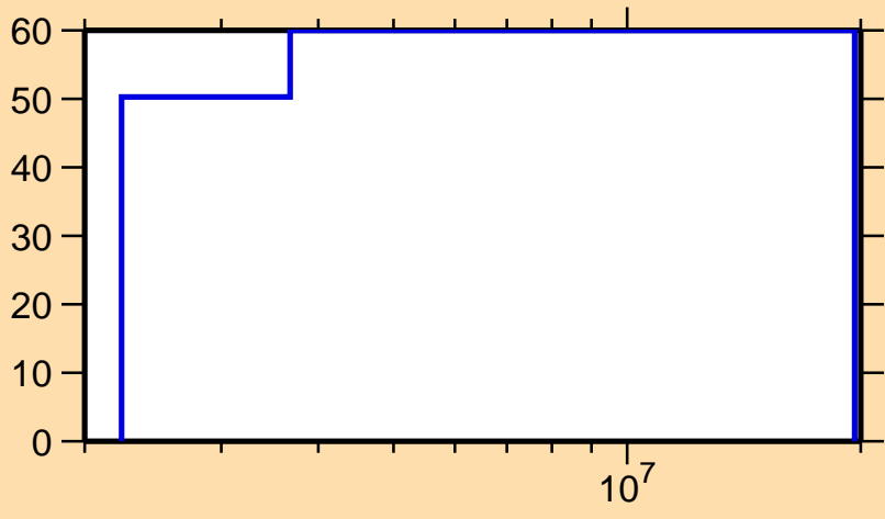
\Delta\sigma/\sigma vs. E for ^{135}\text{Xe}(n,p)
