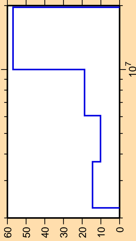
\Delta\sigma/\sigma vs. E for ^{135}\text{Xe}(n,n\text{cont.})
