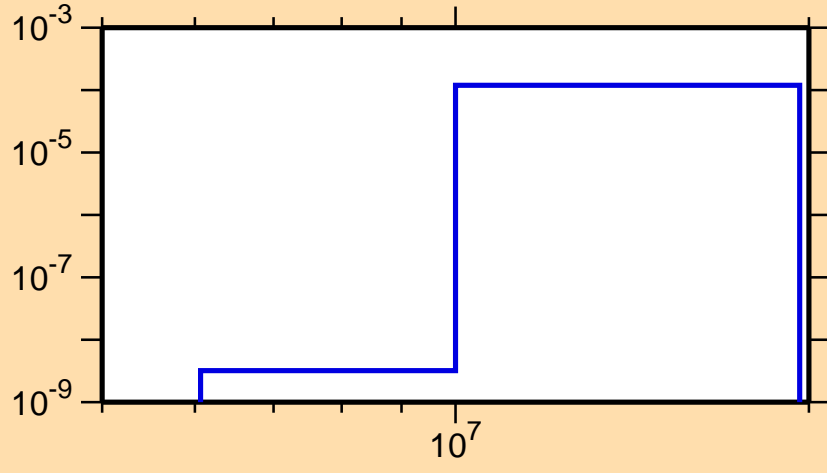
\sigma vs. E for ^{136}\text{Xe}(n,p)
