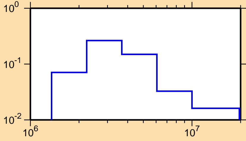
\sigma vs. E for ^{136}\text{Xe}(n,n_2)
