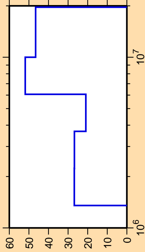
\Delta\sigma/\sigma vs. E for ^{136}\text{Xe}(n,n_2)
