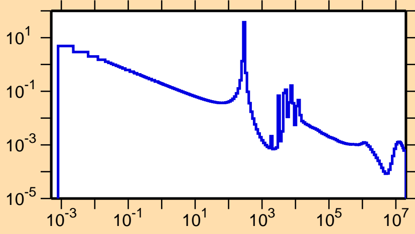
\sigma vs. E for ^{137}\text{Xe}(n,\gamma)
