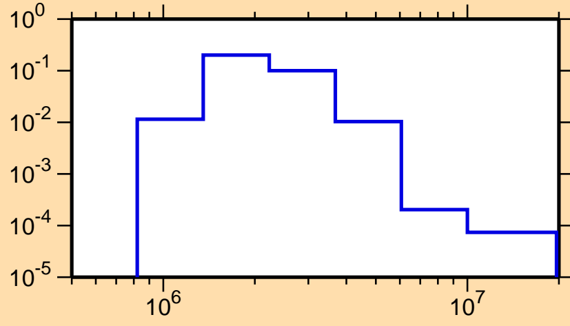
\sigma vs. E for ^{137}\text{Xe}(n,n_3)
