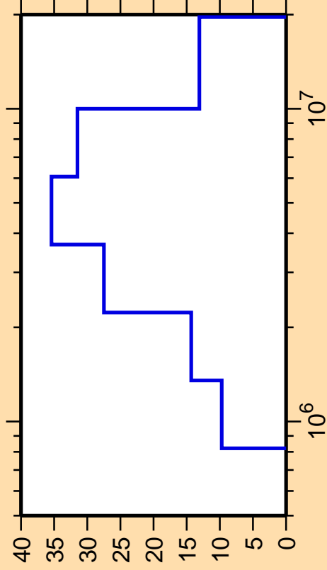
\Delta\sigma/\sigma vs. E for ^{137}\text{Xe}(n,n_3)
