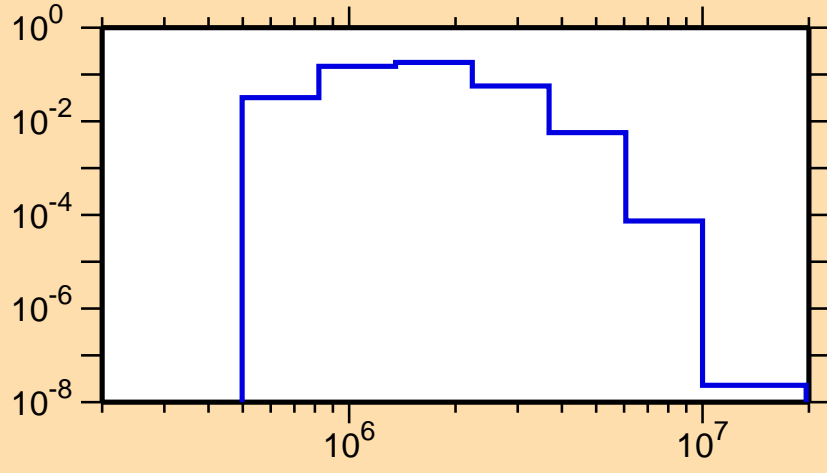
\sigma vs. E for ^{137}\text{Xe}(n,n_1)
