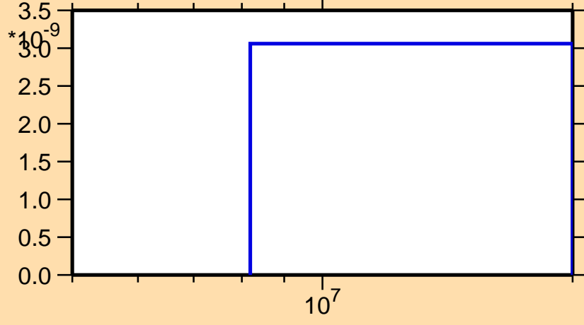
\sigma vs. E for ^{137}\text{Xe}(n,2np)
